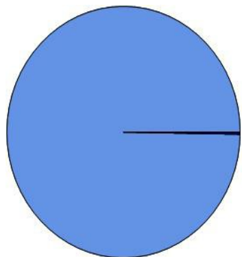
Address Attributes
